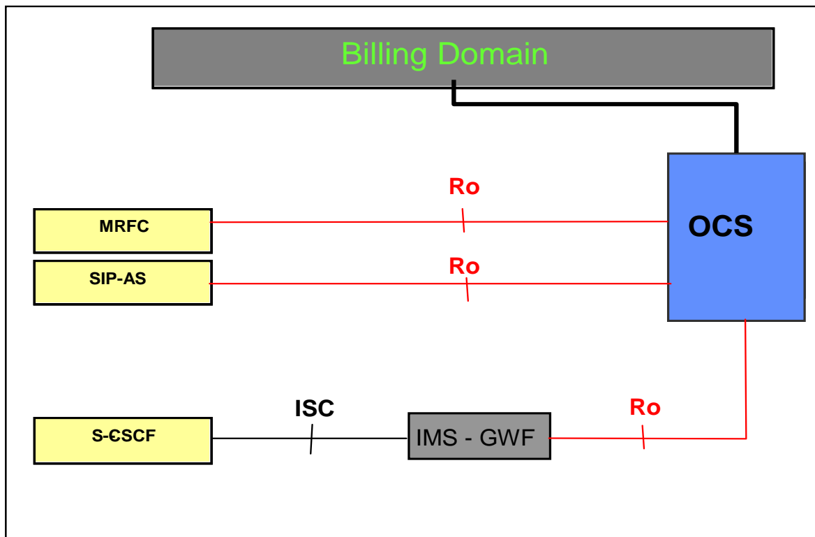
Figure 4.3.1: IMS online charging architecture
