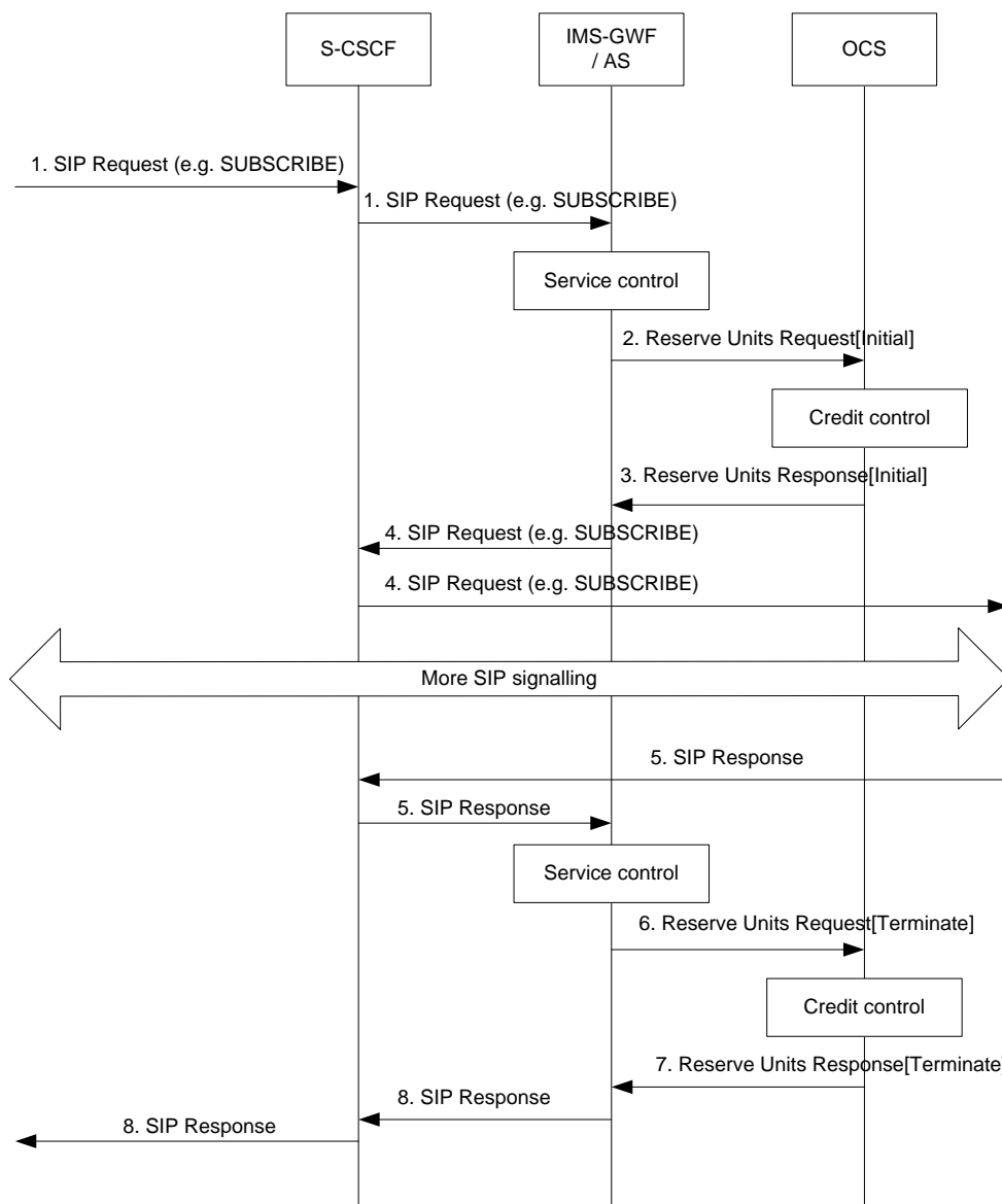
Figure 5.3.2.2.1.3.2.1: Message sequence chart for session-unrelated procedures
