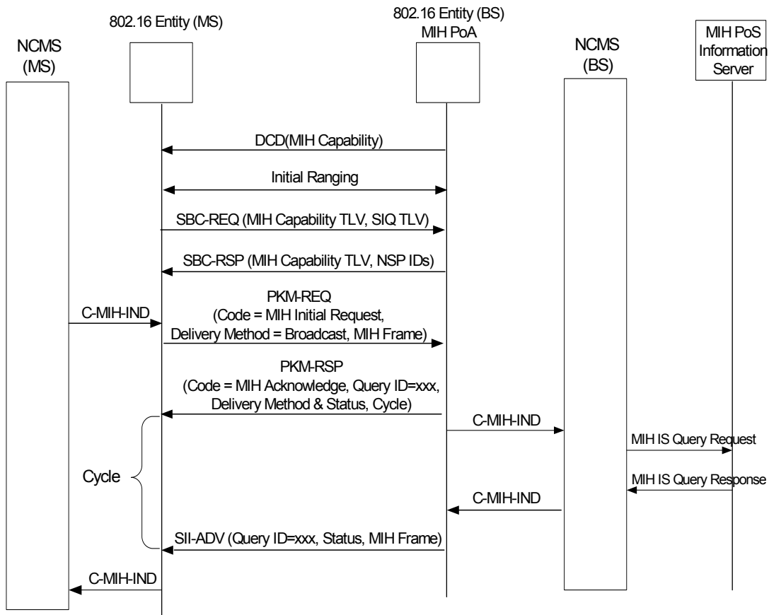
Figure J.11—Pre-authenticated MIH exchange using broadcast delivery method
