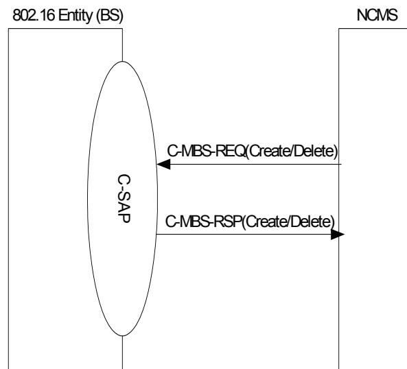
Figure 384—MBS Service Flow (Create and Delete)
