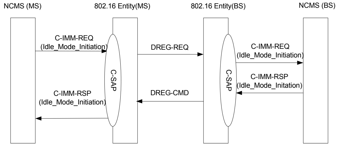
Figure 348—Idle mode initiation (by NCMS on the MS side)
