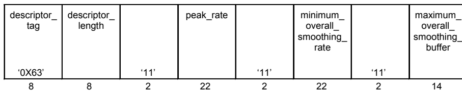
Fig. 9-5 Data structure of partial_transport_stream_descriptor
