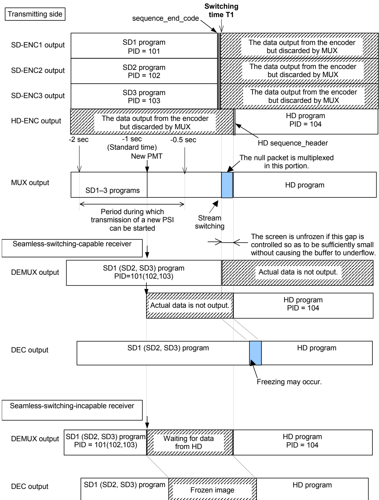
Fig. 1-1 Conceptual diagram of the timing of the transmitting and receiving sides that enables SDTV/HDTV completely seamless switching
