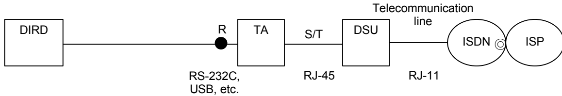
Fig. 9.3.1 R-point connection
