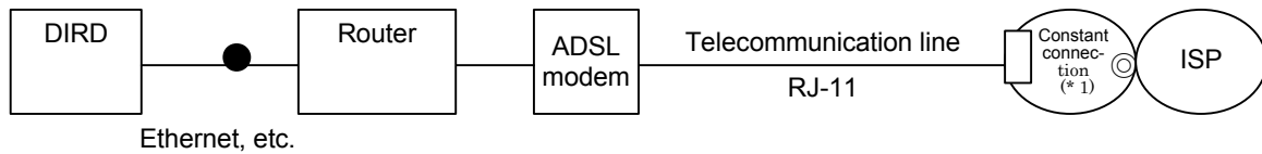
Fig. 9.4.3 Router connection
