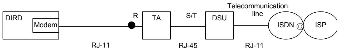
Fig. 9.3.4 TA analog port connection
