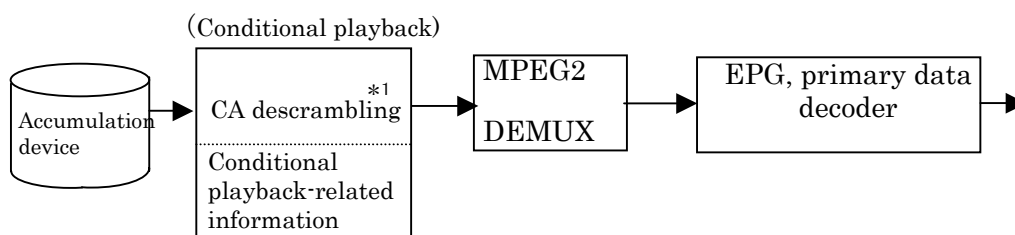
Fig. 11-2-2 Flow of signal processing in service type (2)
