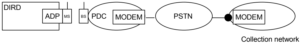
Fig. 9.2.1 PDC-MODEM connection
