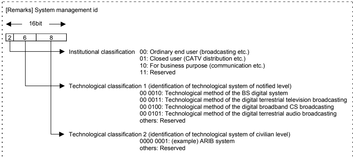
Fig. 13-1 Identification flow of broadcasting/non-broadcasting
