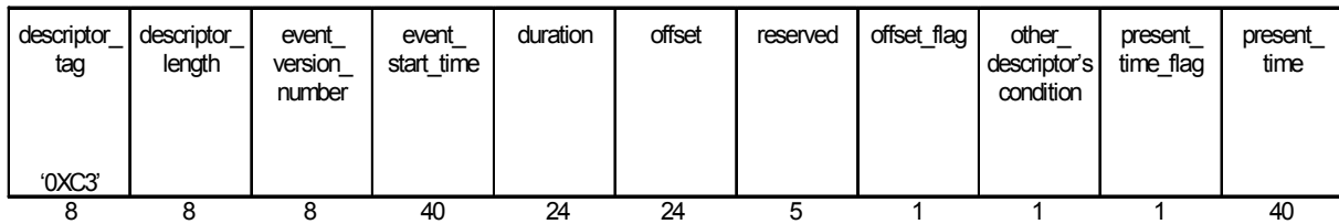
Fig. 9-7 Data structure of partialTS_time_descriptor
