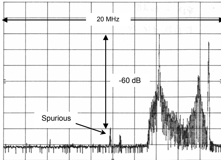
Fig. 1-3 Example of a signal spectrum of an analog television wave with spurious interference
