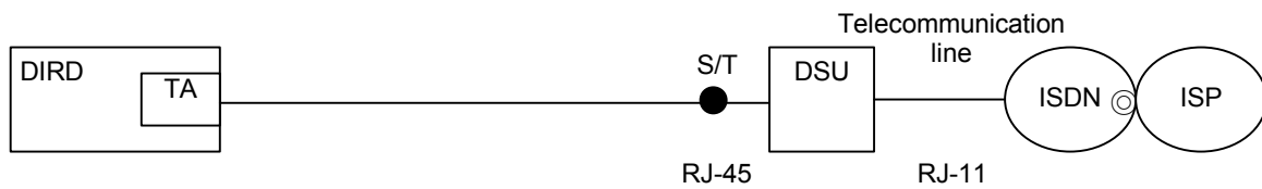
Fig. 9.3.2 S/T-point connection
