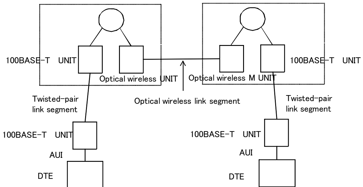
Fig7-1 point to point type typical topology
