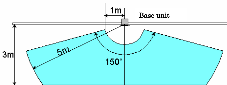
Fig. 3-2 Typical beam profile representation
