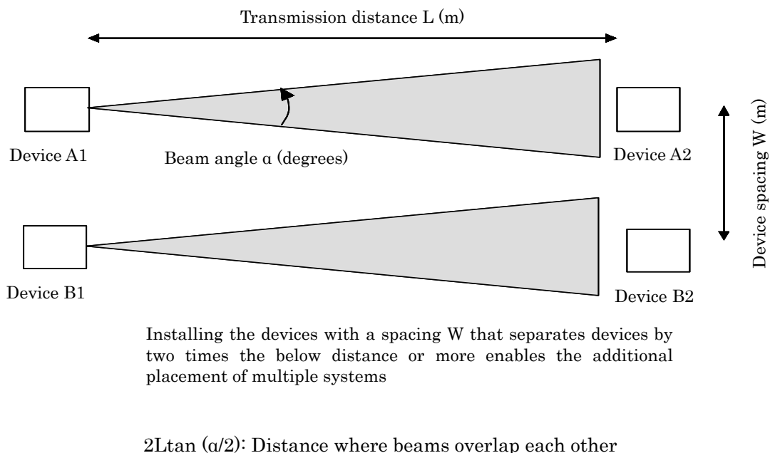
Fig. 11-1 Typical installation of outdoor beam transmission device
