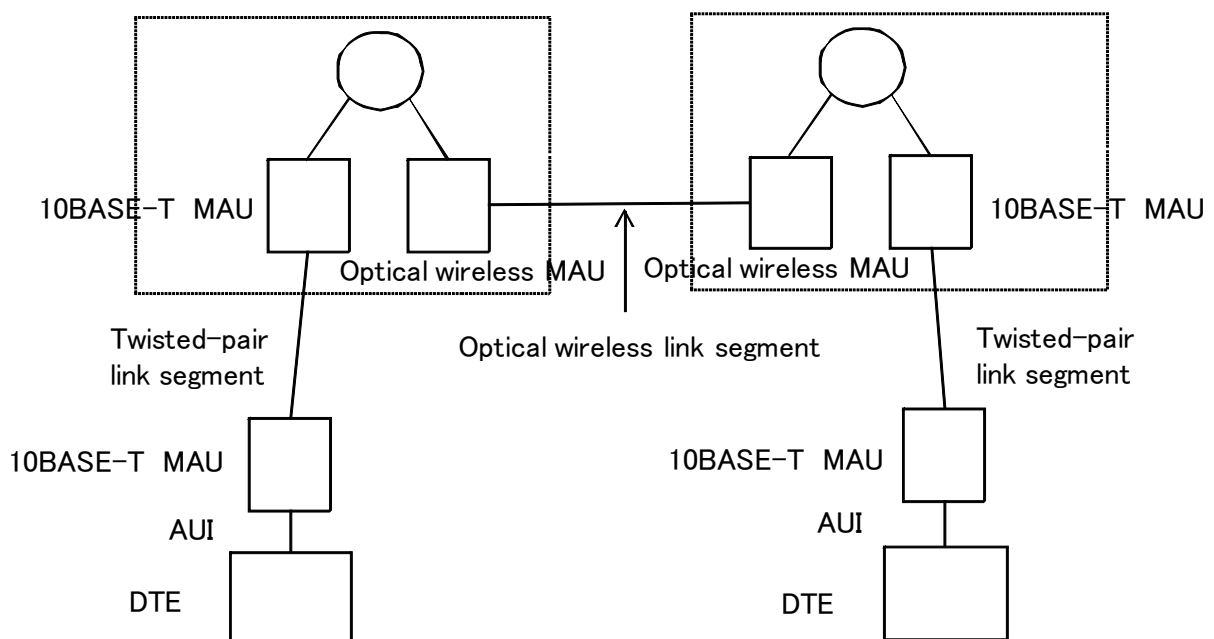
Fig 4-1 point to point type typical topology
