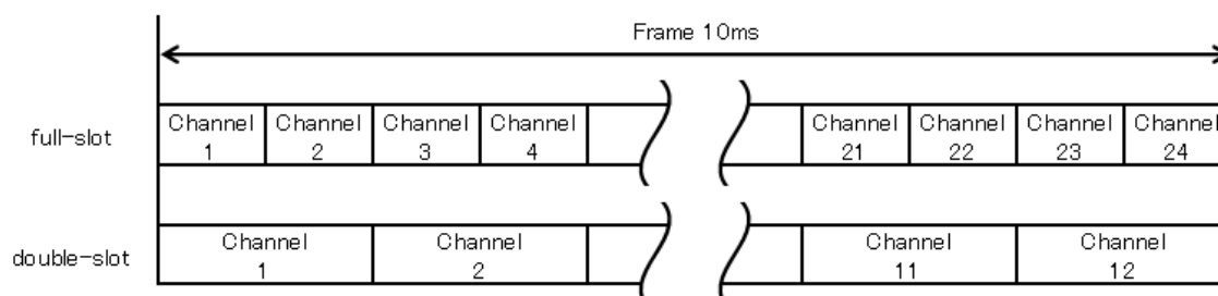
Figure 3-1 Frame Configuration
