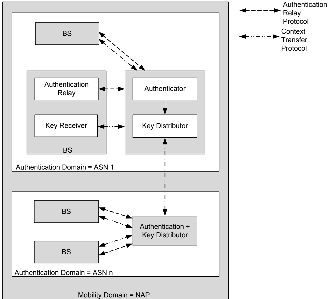
Figure 7-25 - Mobility and Authenticator Domains – Standalone Model
