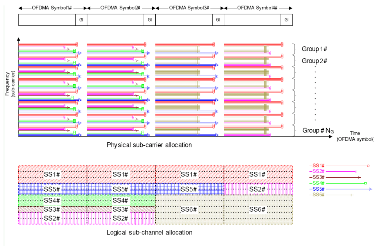
Figure 2-9 Physical and Logical Subchannel allocation
