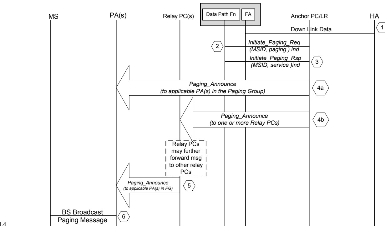
14 15 Figure 7-97 - Paging Generated for MS by Incoming Packets for MS in Idle Mode
