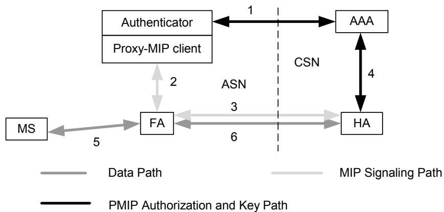
26 Figure 7-76 - PMIP Functional Elements
