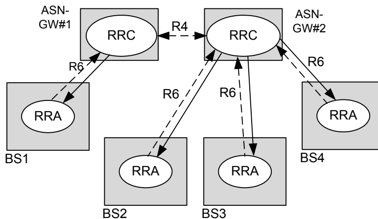
34 Figure 7-88 - RRAs Resident in BS and RRC Resident in ASN
