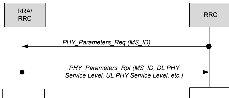
24 Figure 7-92 - PHY Report (Solicited)
