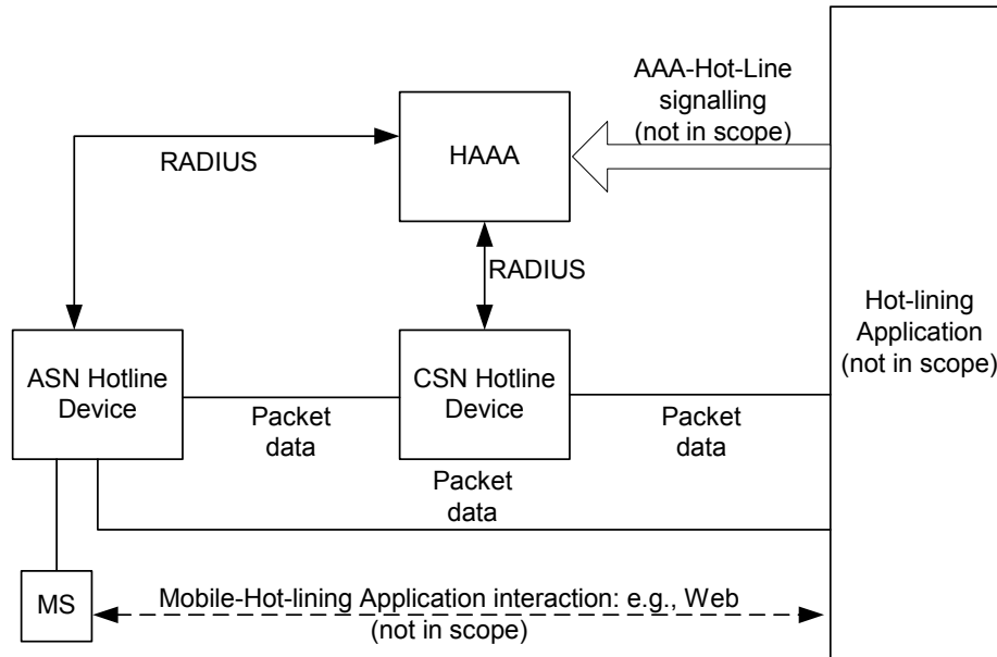
Figure 7-34 - Hot-Lining Operation
