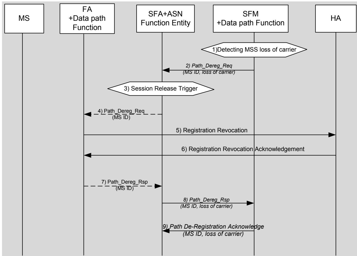
8 9 Figure 7-74 - MS Loss of Carrier Unconventionally Termination
